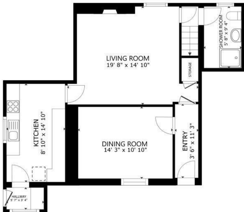
FLOOR 1
